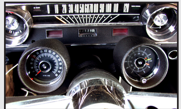
Figure 2: Rally Pac positioned and mounted
