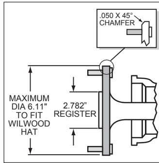
Figure 3. Axle Flange Maximum Dimension
