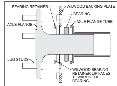
Figure 4. Retainer / Axle Diagram
