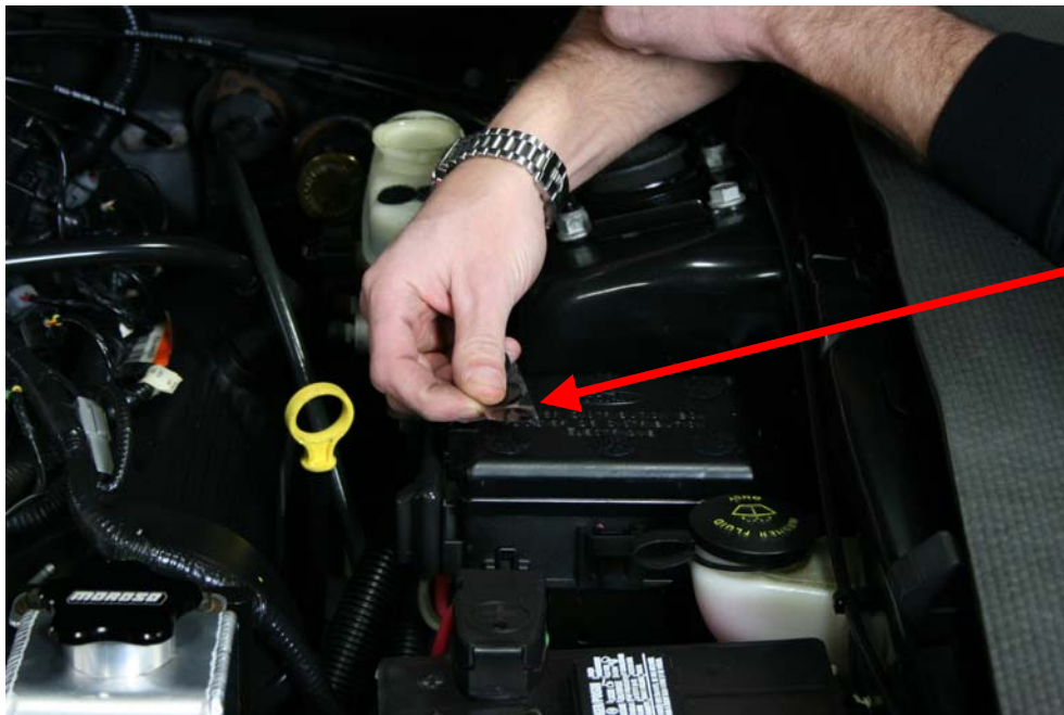
Step 2: Secure Velcro loop dots to each dot previously installed
