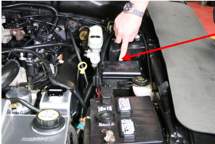
Step 1: Locate fuse box and install Velcro hook dots as shown 6 places
